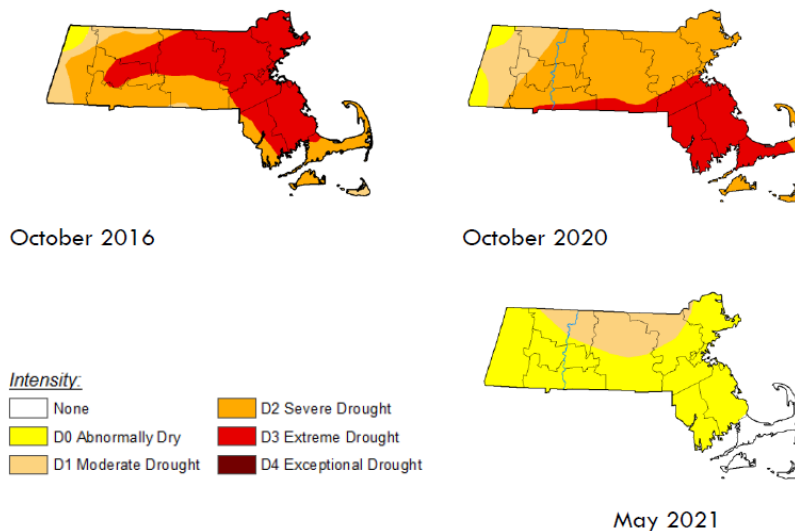
Figure 13: Recent Massachusetts Drought Events (2016-2021)
