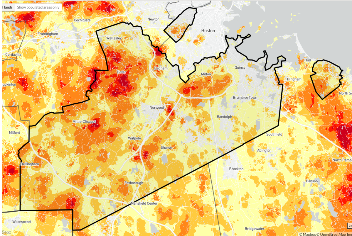
Figure 24: Wildfire Risk Areas in Norfolk County
