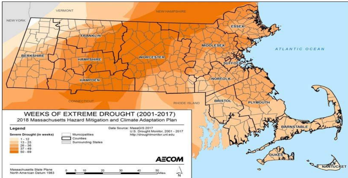
Figure 12: Weeks of Extreme Drought (2001-2017)
