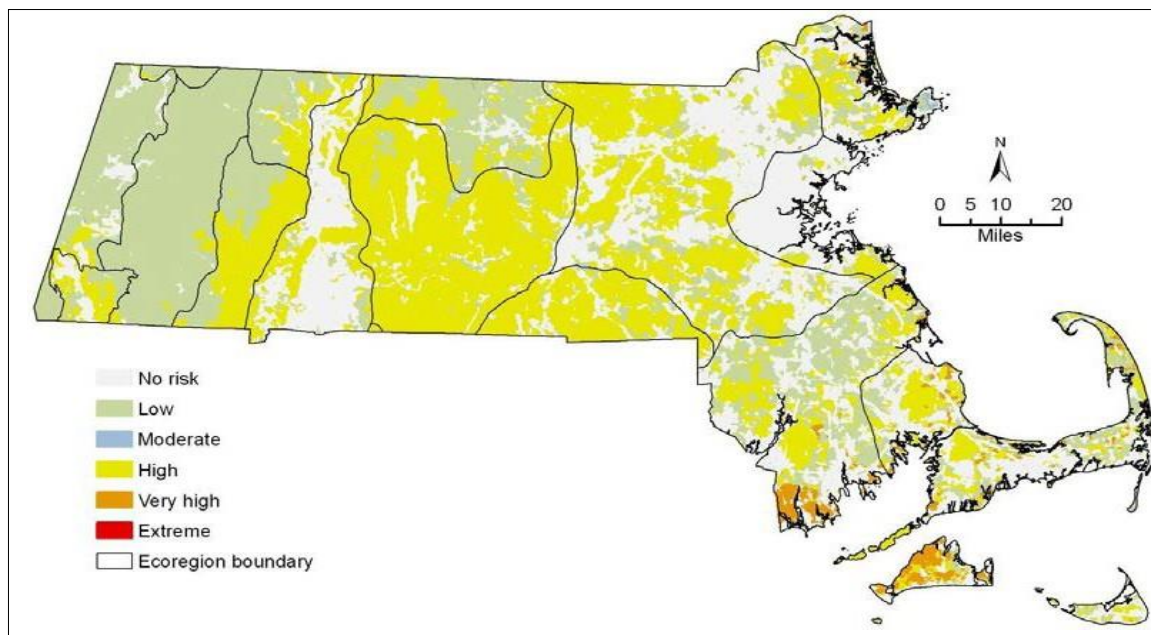
Figure 23: Wildfire Risk Areas in Massachusetts
