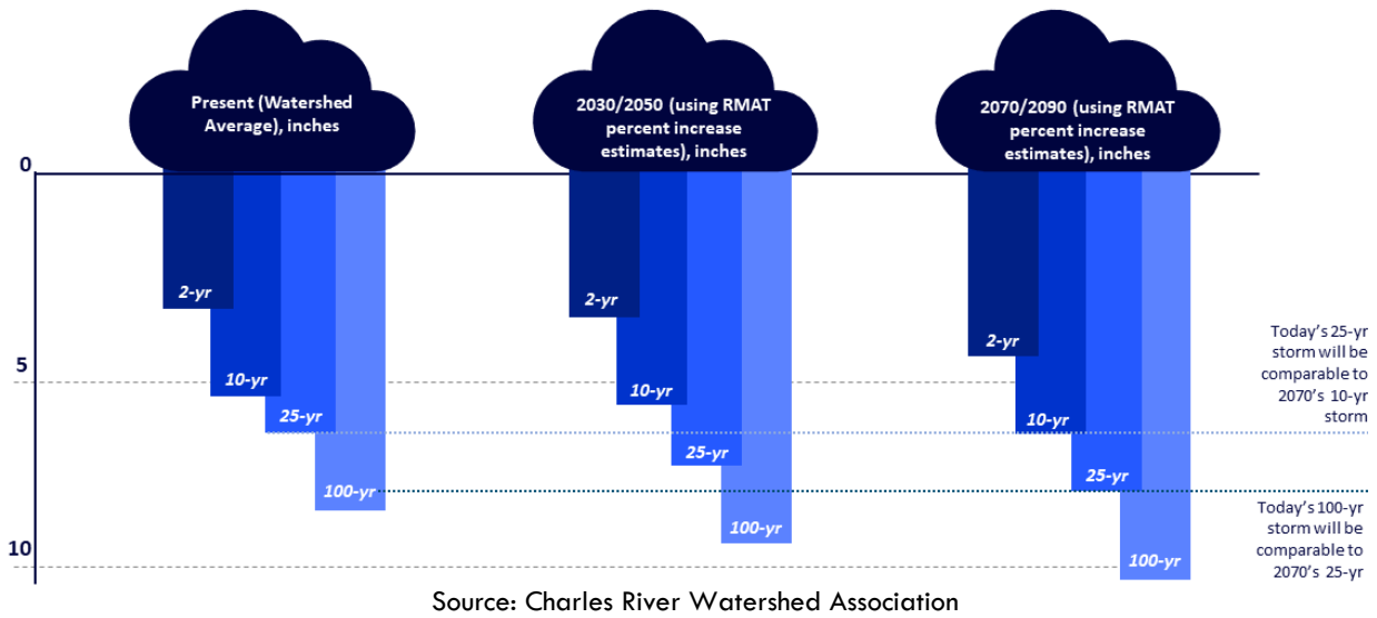
Figure 10: Projected future increase in precipitation scenarios in the Charles River Watershed Model
