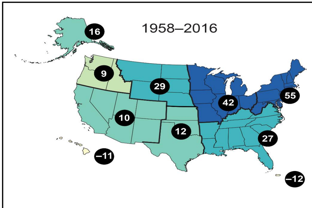
Figure 4 Observed Change in Total Annual Precipitation Falling in the Heaviest 1% of Events
