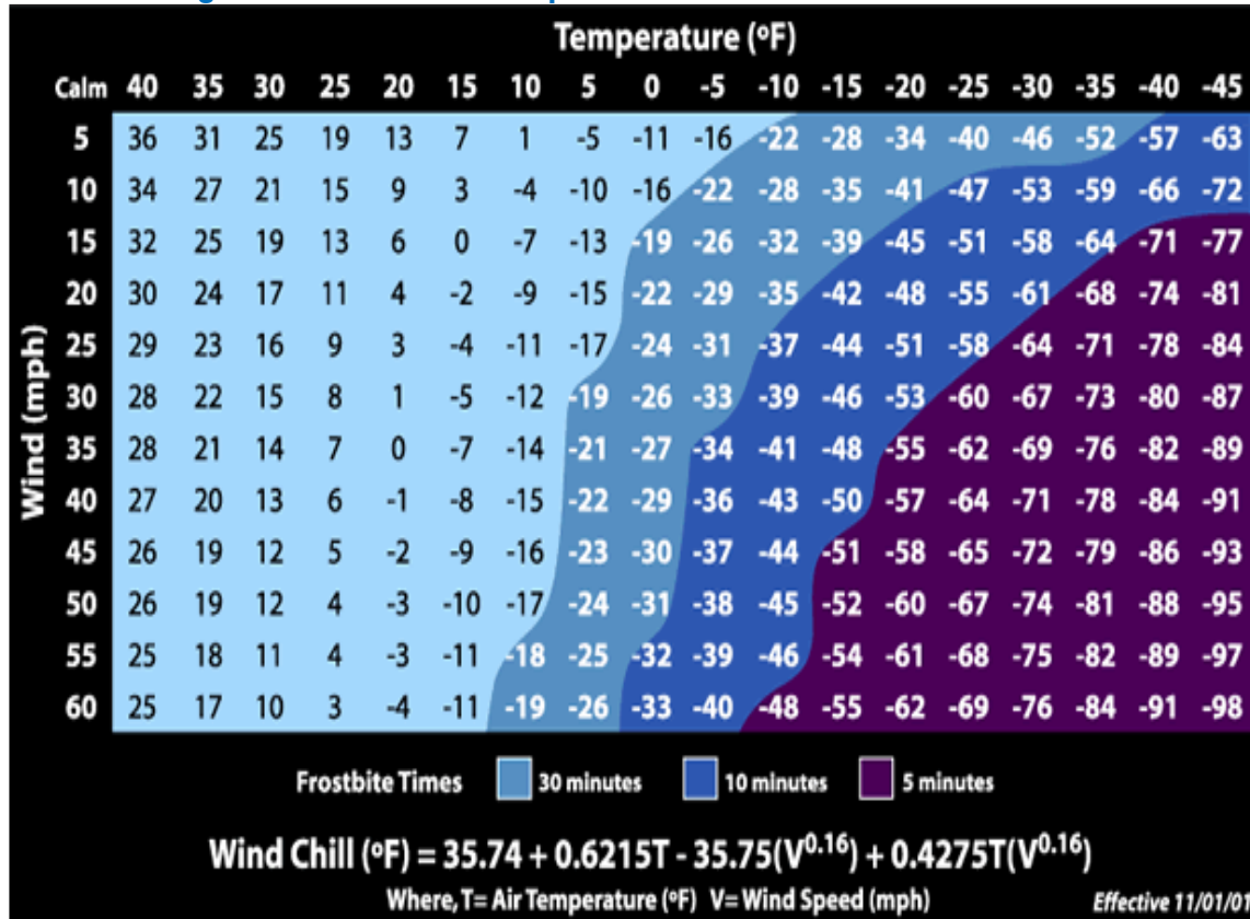
Figure 17. Wind Chill Temperature Index and Frostbite Risk
