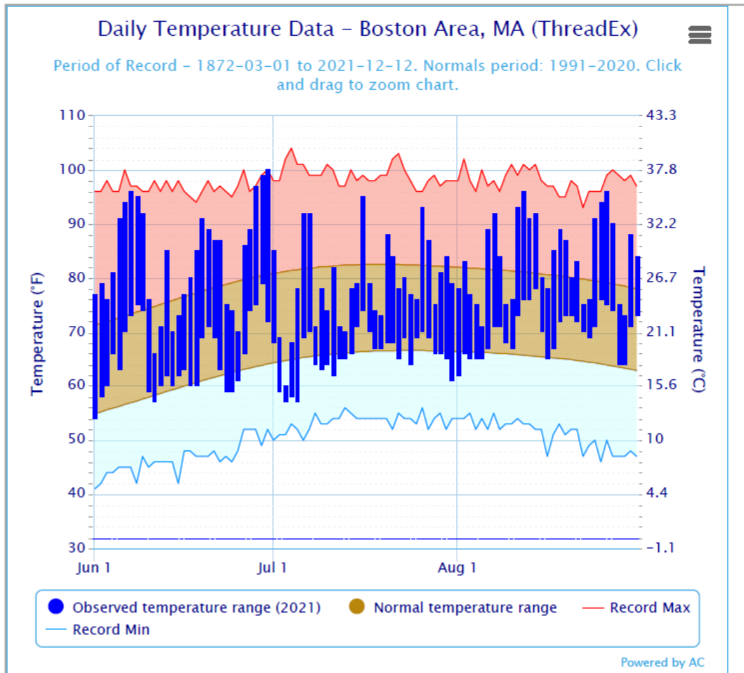
Figure 20: Summer 2021 Temperatures, Boston Area
