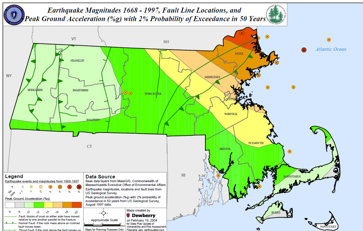
Figure 26: Massachusetts Earthquake Probability Map
