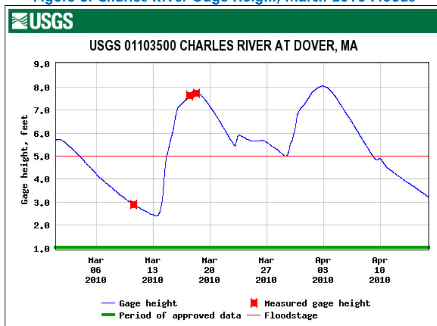
Figure 8: Charles River Gage Height, March 2010 Floods
