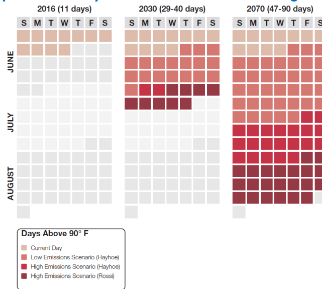
Figure 22: Comparison of Days Above 90F for Low and High Emission Scenarios
