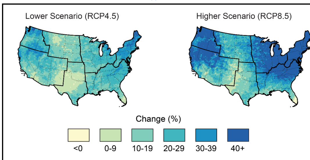
Figure 5: Projected Change in Total Annual Precipitation Falling in the Heaviest 1% of Events for 2070-2099
