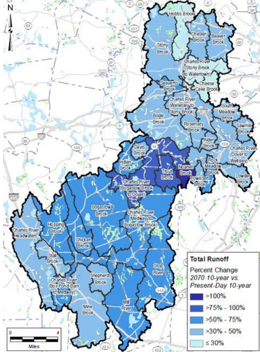
Figure 11: Percent increase in total runoff volume during the 2070 10-year event versus the baseline 10-year event, by sub-basin
